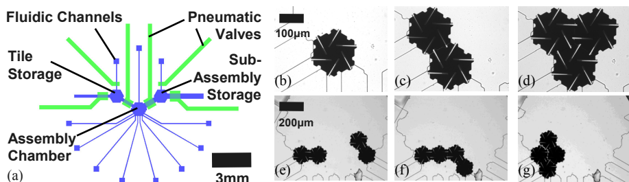
Figure 2. Multi-Chamber Microfluidic Assembly Chip and Assembly Component Designs (a) Multilayer PDMS chip design allows on-chip valving to isolate three separate chambers. The left chamber is used to select and store good quality tiles to be assembled in the main assembly chamber (centre). The right chamber is used to store sub-assemblies for hierarchical assembly. (b-d) Assembly of two- and three-component structures. (e-g) Hierarchical assembly experiments.
