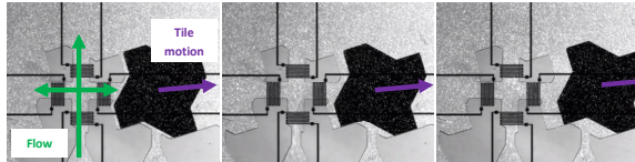
Sequence 2: Heater off, viscosity valve opens, mobile tile rejected from structure.
